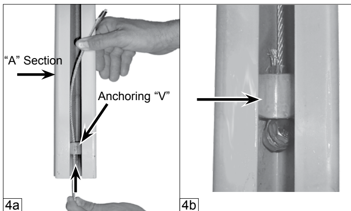
4a. Feed the crimped end of the new cable through the "A" section anchoring "V" from the bottom as shown. 4b. Make sure the anchoring end of the cable is pulled snugly against the anchoring "V" as shown. (NEVER DISASSEMBLE THE NUT AND BOLT OF CABLE ANCHORING ASSEMBLY)
