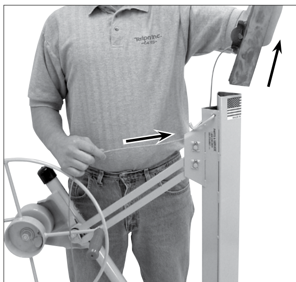
3. Remove the two telescoping sections completely from the frame housing. Pull the cable completely out from the frame along with them. BE CAREFUL for loose strands or frays on the cable.
